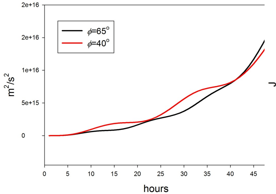
Total kinetic energy, \text{m}^2/\text{s}^2
