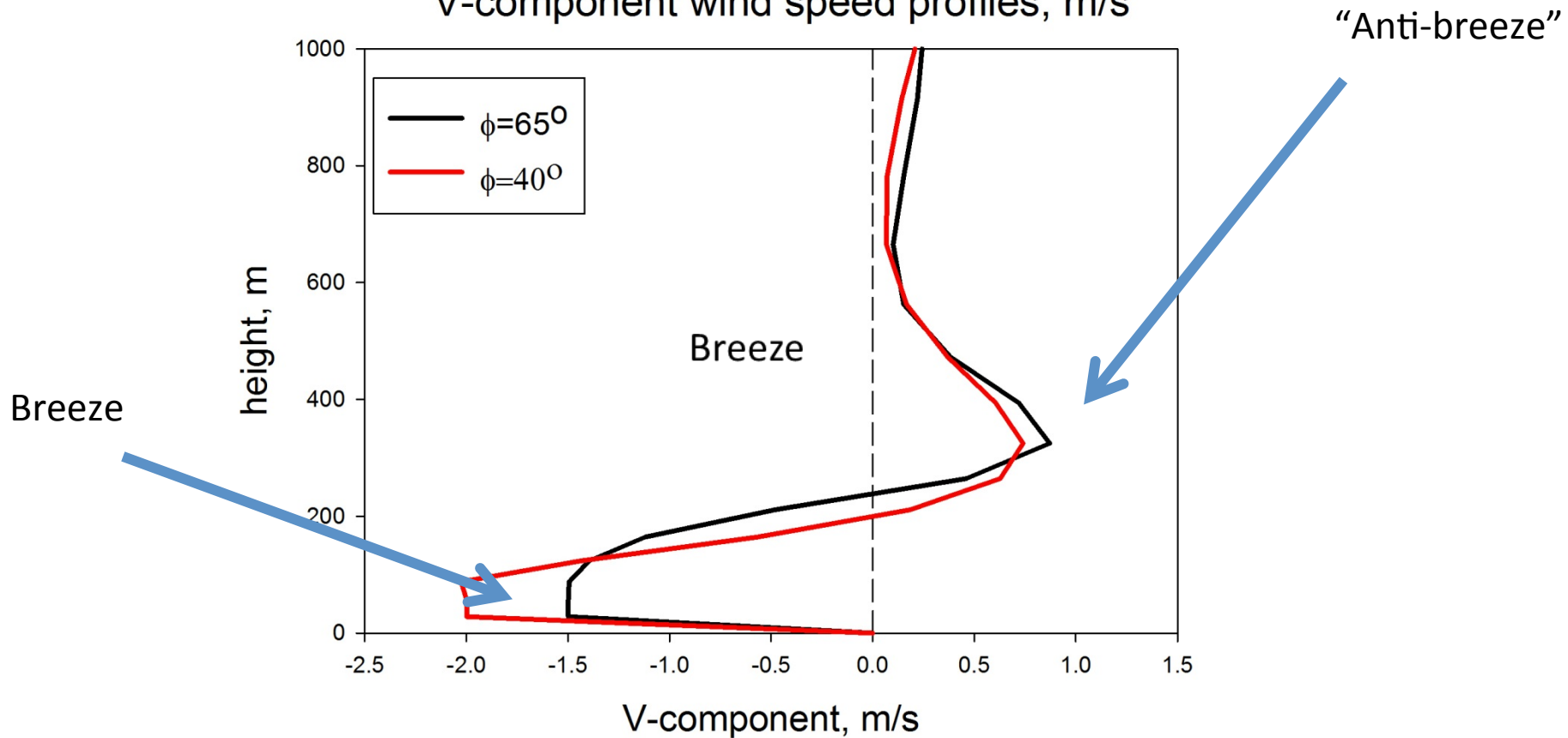
V-component wind speed profiles, m/s
