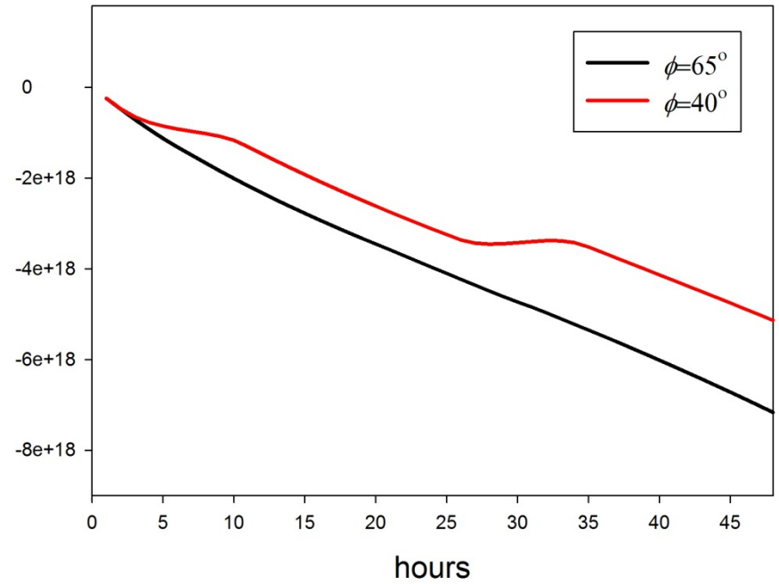
Perturbation potential energy, J
