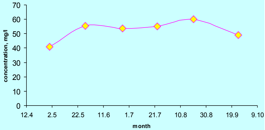
Dynamics of carbon concentration in bog water
