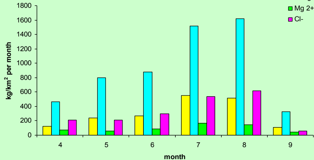
Dynamics of ions flow in a river basin
