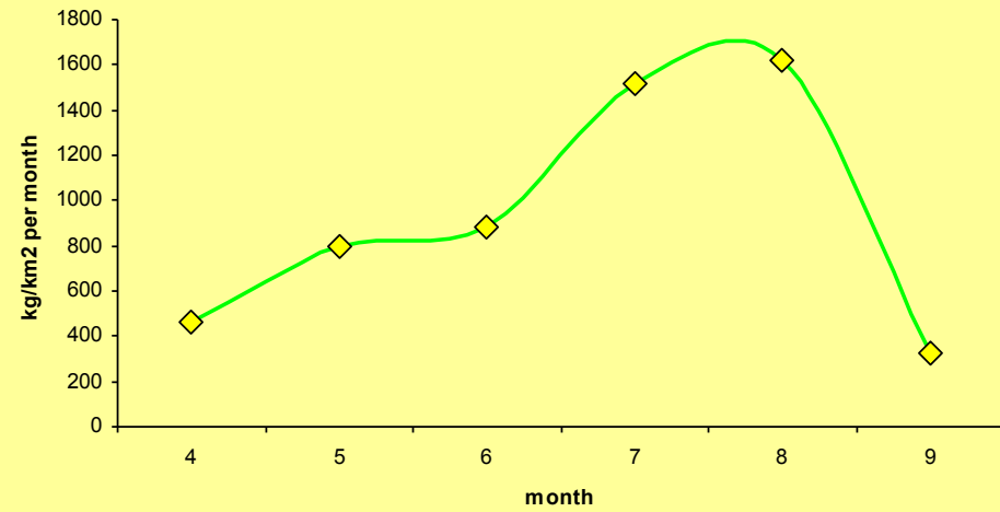
Carbon flow from the river basin
